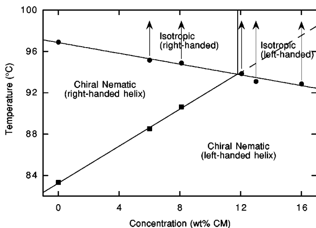
FIG. 2. Phase diagram of the CM-EPHDBPE system. filled circles: chiral nematic-isotropic transition. filled squares: helix inversion. The lines are linear least square fits to the data. The arrows denote where optical activity measurements were made. The helix inversion line is vertical in the isotropic phase.
